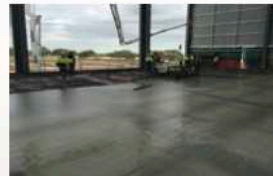
Somero S485 Laser Screed
